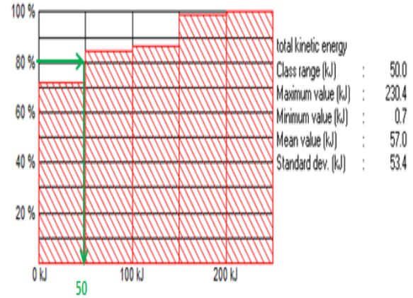
Figure 9. Histogram kinetic energy of rock blocks banging the rockfall barriers. Source: Data Analyses, 2013
