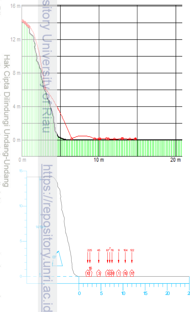
Figure 3. Simulated the rockfall travel modes and Kloch Slope Source: data simulation and private documentation, 2011
