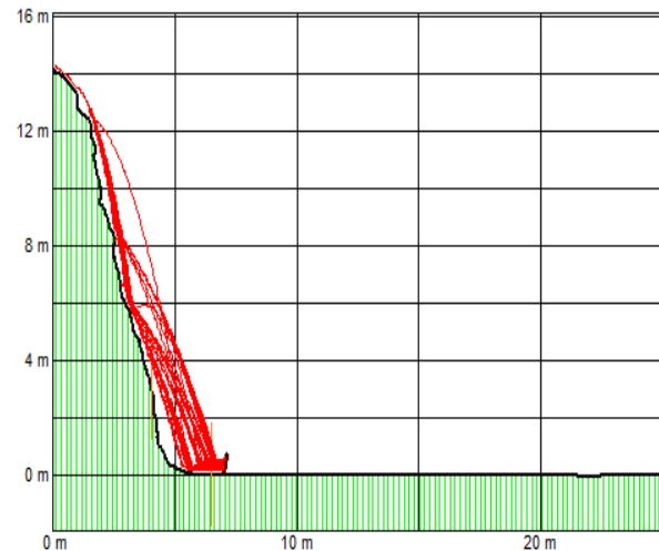
Figure 10. Rockfall risk zones. Source: Data Analyses, 2013
