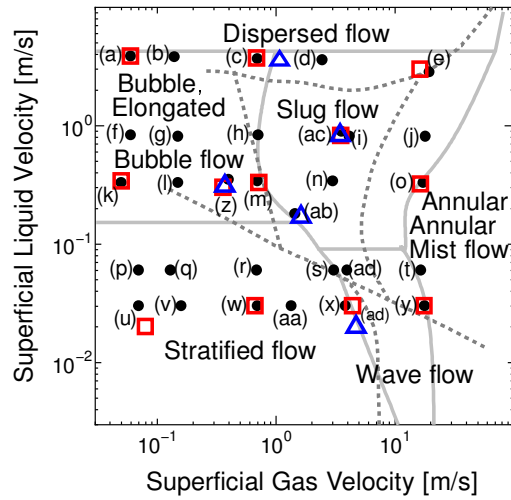
(a) Mandhane [10] and Baker [11] Maps for Horizontal Flow.
