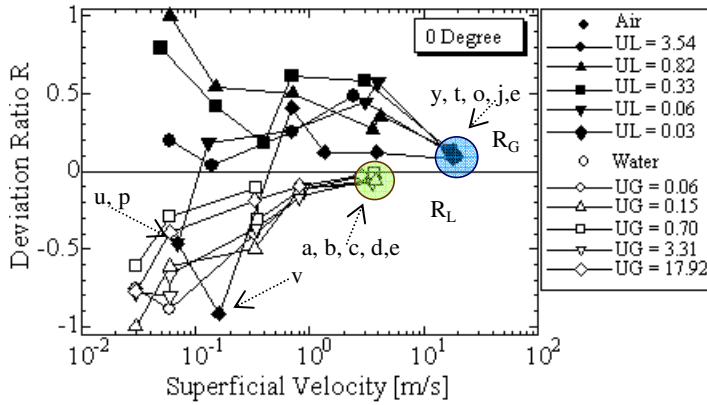
(a) Superficial Velocity on Deviation Ratio.
