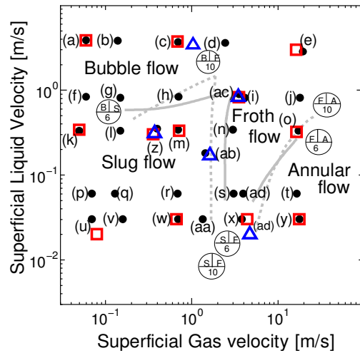
(b) Sekoguchi [12] Map for Vertical Flow.
