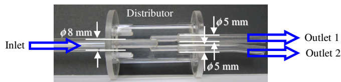
Fig. 3. Distributor.
