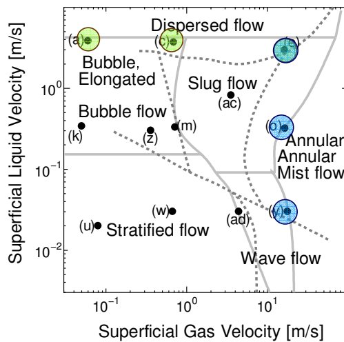
(b) Map [10, 11] for Horizontal Flow.
