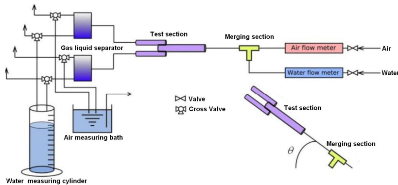
Fig. 1. Experimental Apparatus.
