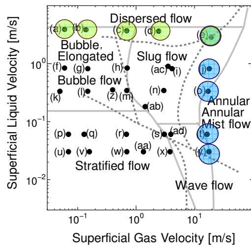
(b) Mandhane [10] and Baker [11] Map for Horizontal Flow.
