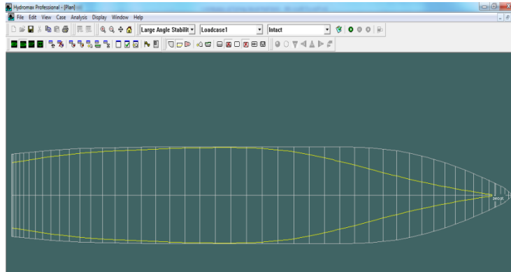
Figure 5. (A) Waterplane area of displacement hull
