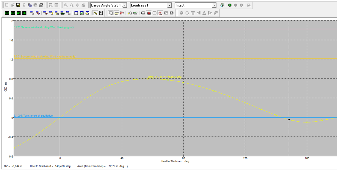
Figure 6. GZ curve for each vessels
