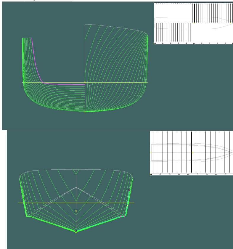
Figure 4. Body plan of displacement hull and planning hull
