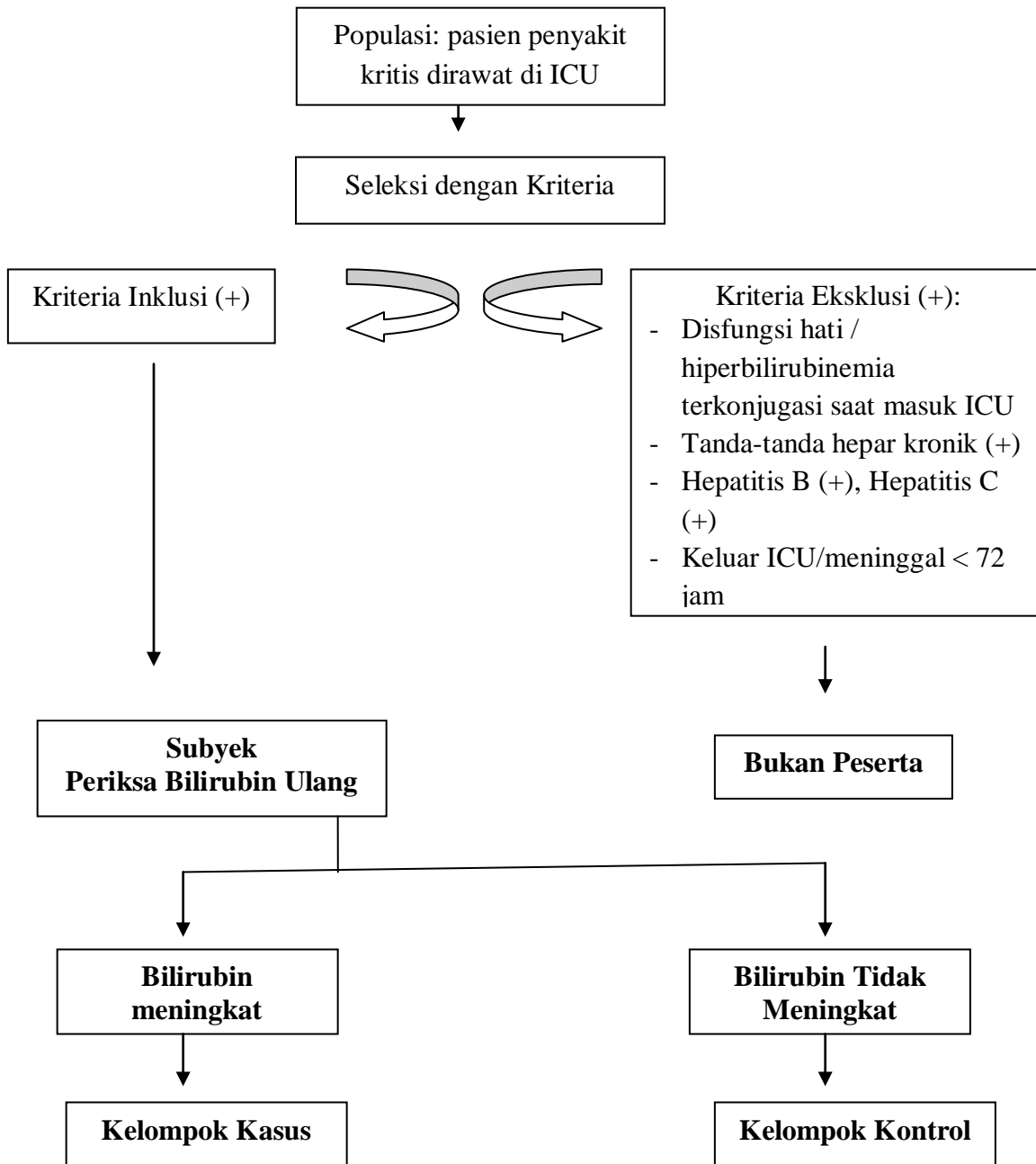
Gambar 3. Alur Penelitian
