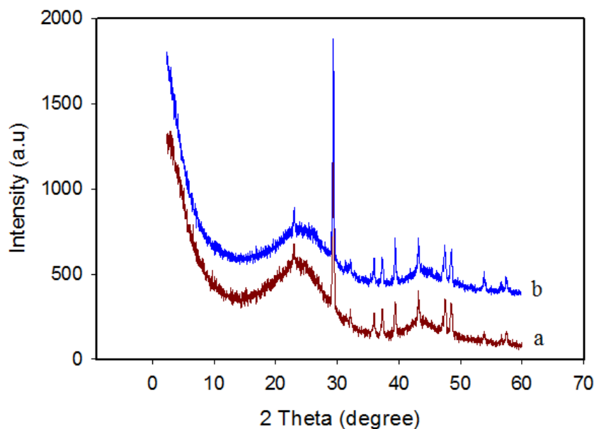
Figure 3. XRD patterns of ACM2 and ACM4 activated for 2 (a) and 4 (b) hours, respectively.
