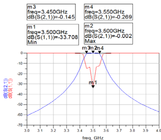
Gambar 11. Hasil simulasi Band Pass Filter berdasarkan S-parameter
