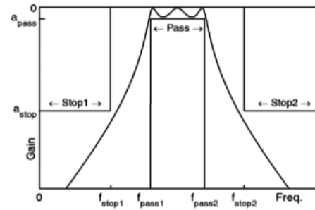
Gambar 6. Respon Filter BPF
