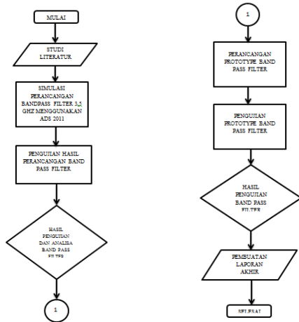
Gambar 10. Diagram Alir Desain Band Pass Filter
