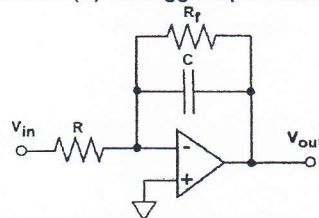
Gambar 3. Rangkaian inverting integrator [10]
