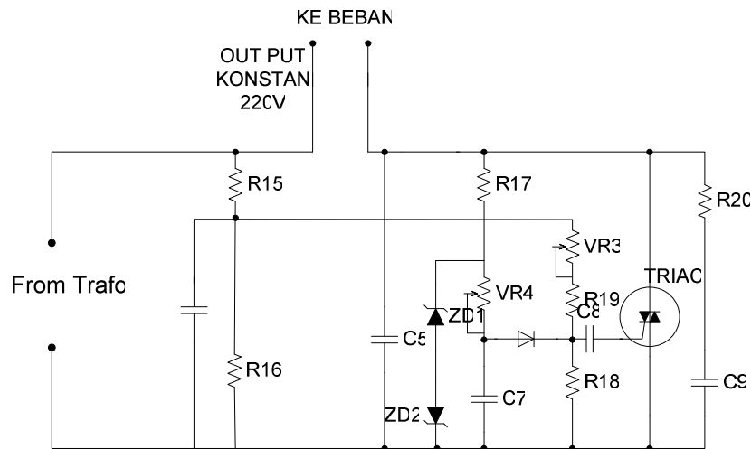
Gambar 5. Rangkaian Penstabil (Anonim, 1990)
